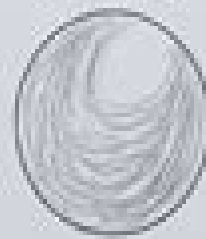
Contour
