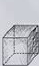
Hatching
