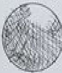
Cross-Hatching
