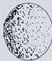
Stippling
