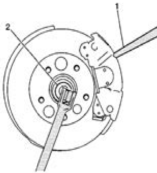
Fig. 3: Preventing Rotor Turning Using Drift Or Punch Courtesy of GENERAL MOTORS CORP.
