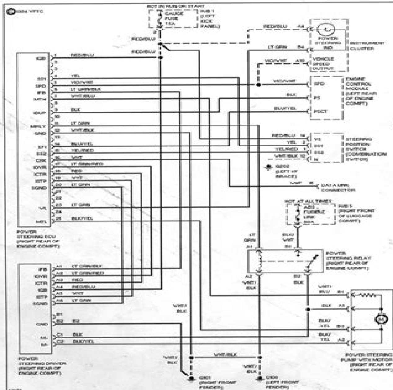
Electronic Power Steering Circuit
