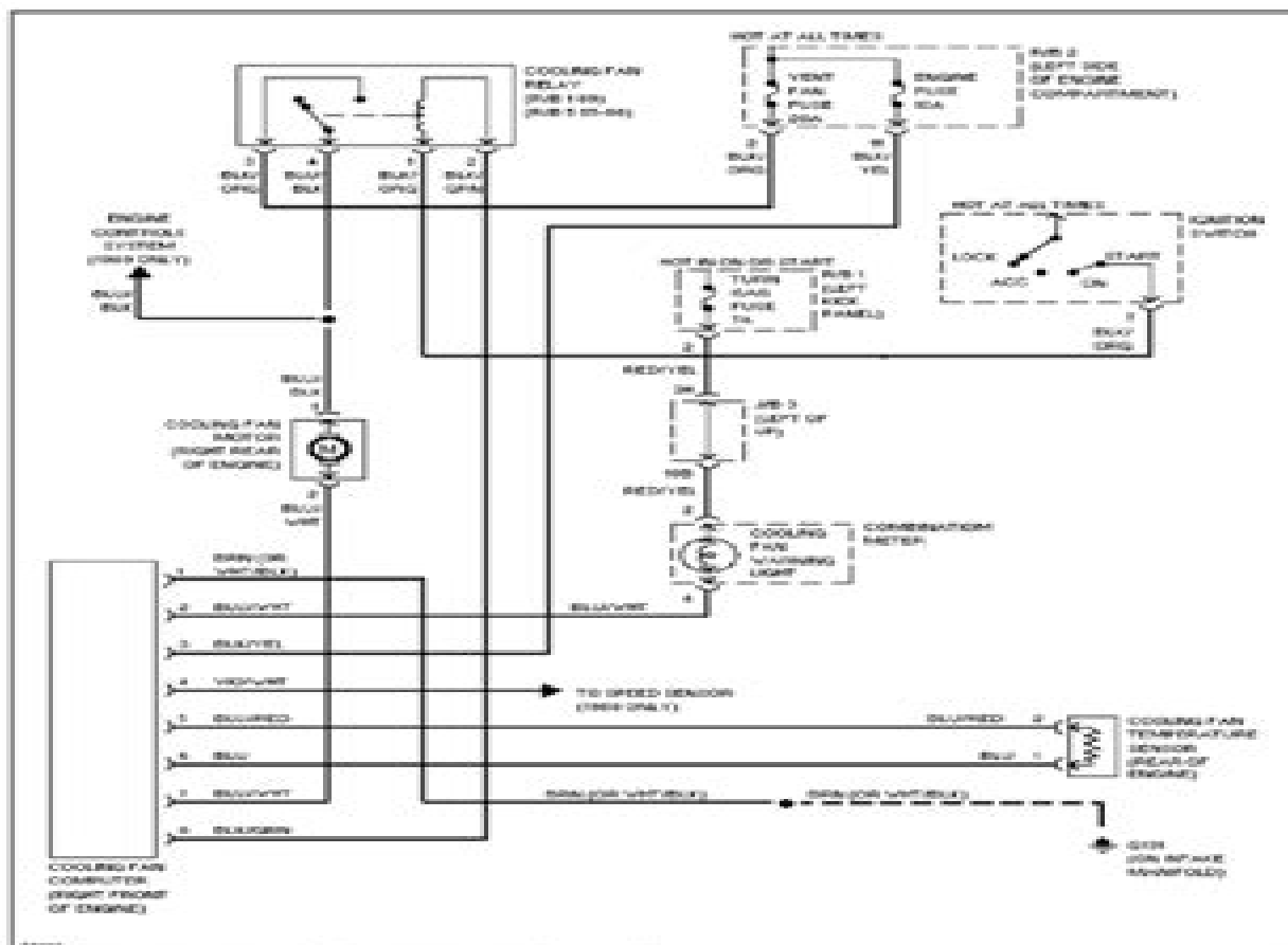
Engine Compartment Cooling Fan Circuit
