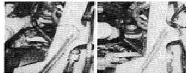
Disconnecting the Brake Wire Bracket LH SAG9-31, 32
