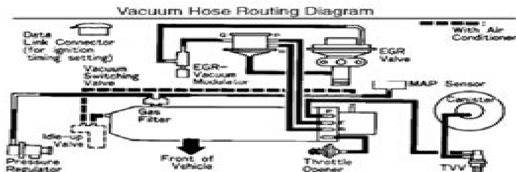
Fig. 1: Vacuum Diagram (Camry 2.2L)
